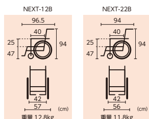
NEXT-12B (自操式)
