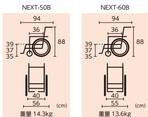
NEXT-50B (自操式)
