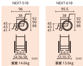
NEXT-51B (自操式)
