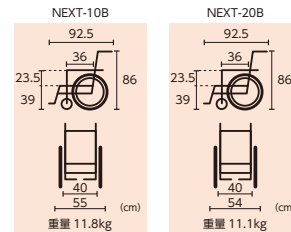
NEXT-10B (自操式)
