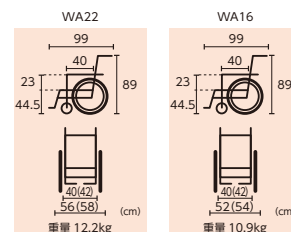
WA22 (自操式)
