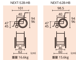
NEXT-52B-HB (自操式)
